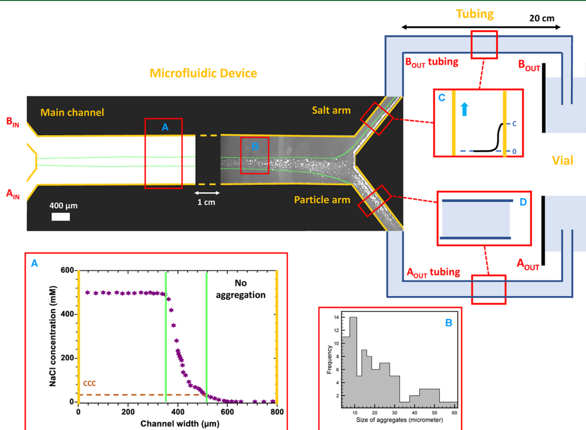
Figure 4. MD experiment. (Top left) Image of the main straight part of the MD and the two outlet arms. Tubing connects the outlet to the vial. (A) Salt concentration profile along the width of the MD. The two yellow and green lines (color online) correspond to the lateral walls of the MD and to the SG in which the salt concentration is higher than the CCC, respectively. (B) Size distribution of the aggregates deposited on the top wall of the MD. (C) Concentration profile of the nanoplastics in the B_{out} arm and tubing. (D) Image of the colloidal deposit in the A_{out} arm and tubing. The blue arrows in 1 and 3 indicate the flow direction.
