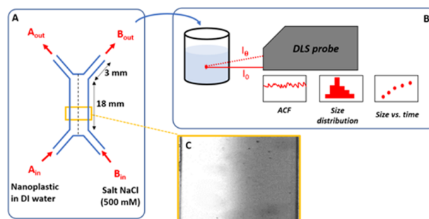
Figure 2. (a) Sketch of the experimental conditions in the MD. After the nanoplastics flow through the MD, they flow through the tubing and are eventually collected in vials. (b) DLS allowed us to determine the evolution of the aggregate size over time. (c) View of the interface between the nanoplastic suspension (left) and a patent blue V dye suspension with the same diffusion coefficient as that of the saline suspension. The variation in the gray level across the channel allowed us to determine the salt concentration profile averaged over the height of the MD after a calibration experiment. This profile image is from an experiment with Q = 2 \text{ mL h}^{-1} and was taken in the middle of the straight part of the MD.
